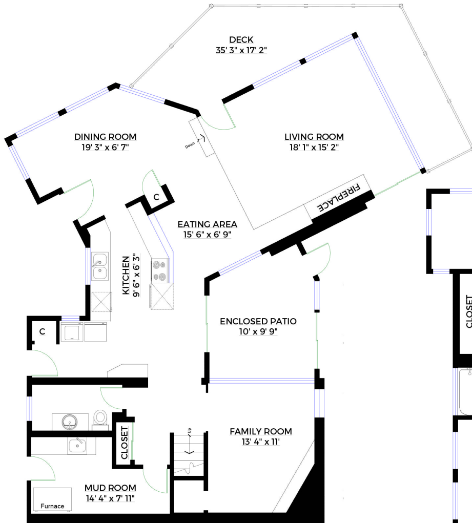
MAIN LEVEL Floor Area: 1,279 Sq. Ft.
